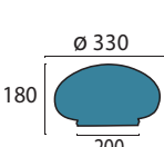
Glas 330 champ matt Ø 330 mm, H 180 mm champagne matt Griffrand 200 mm
