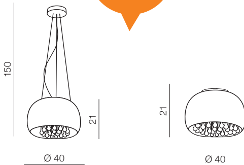
Burn AZ0699 PENDANT/TOP 5x G9 Only LED metal/glass/crystal chrome/chrome/clear
