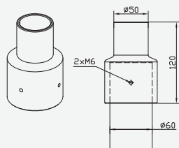
Art. 3060 Reduction for ø50mm fittings for mounting on a ø60mm pole
