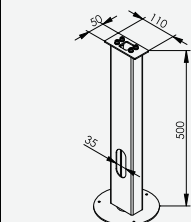
Art. 1907 Concreting anchor Art: 1311, 1312 Art: 1901
