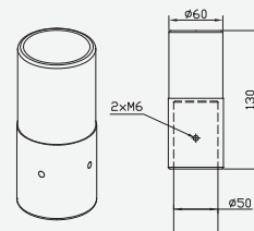
Art. 3070 Reduction for ø60mm fittings for mounting on a ø50mm pole
