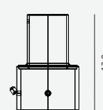
Art. 7660 Reduction for ø60mm fittings for mounting on a ø76mm pole, to be used with Visby and Koster luminaires
