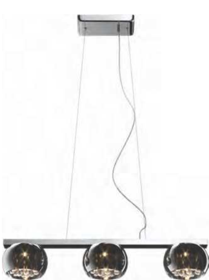
4. CRYSTAL | Pendant lamp P0076-03S-F4FZ 3 x G9 MAX 42W smoky chrome glass shade clear crystal drops inside
