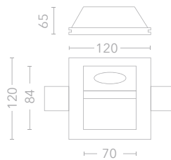
CUT OUT 126x123mm
