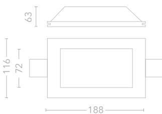
CUT OUT 118x191mm
